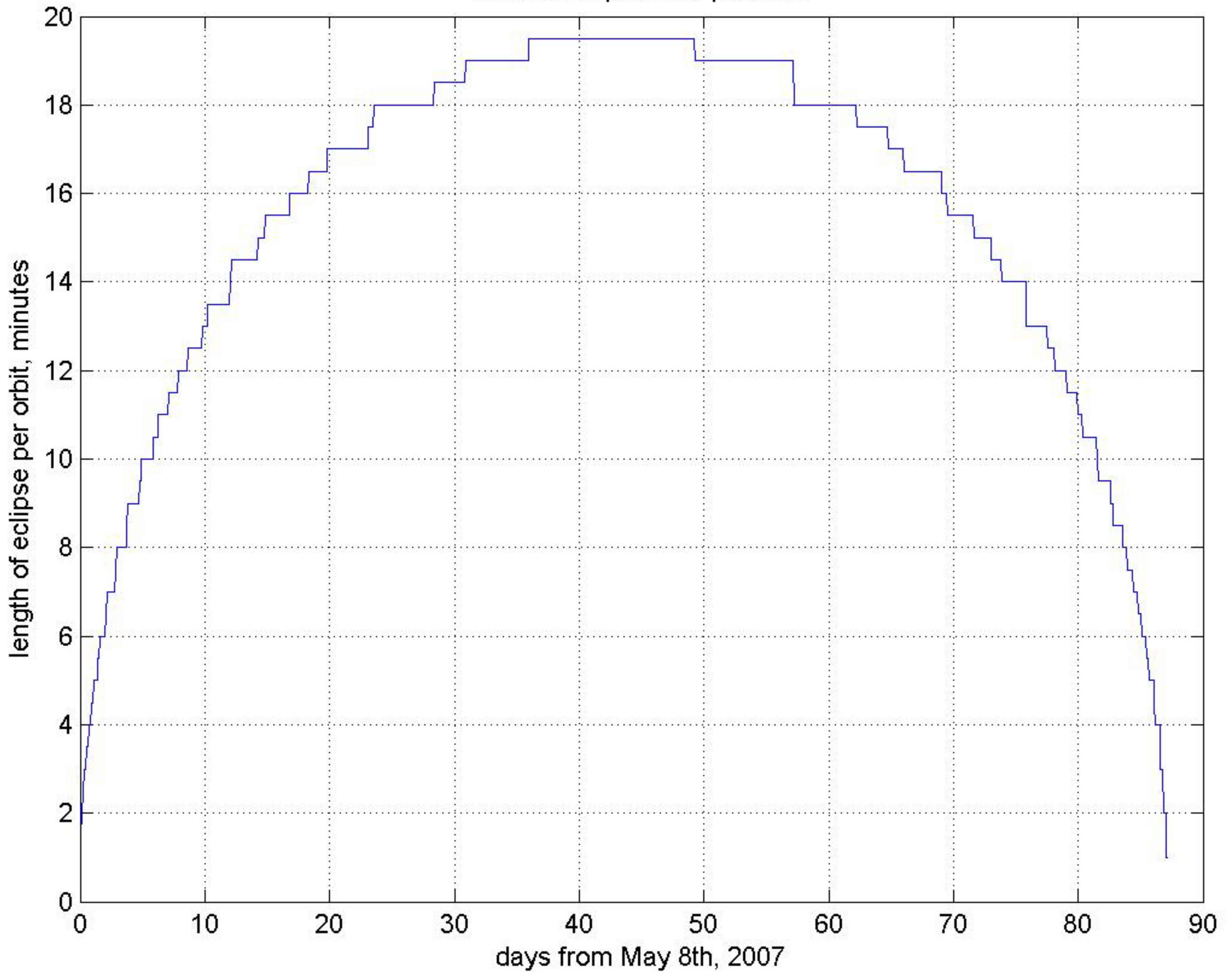
Hinode Eclipse time per orbit
