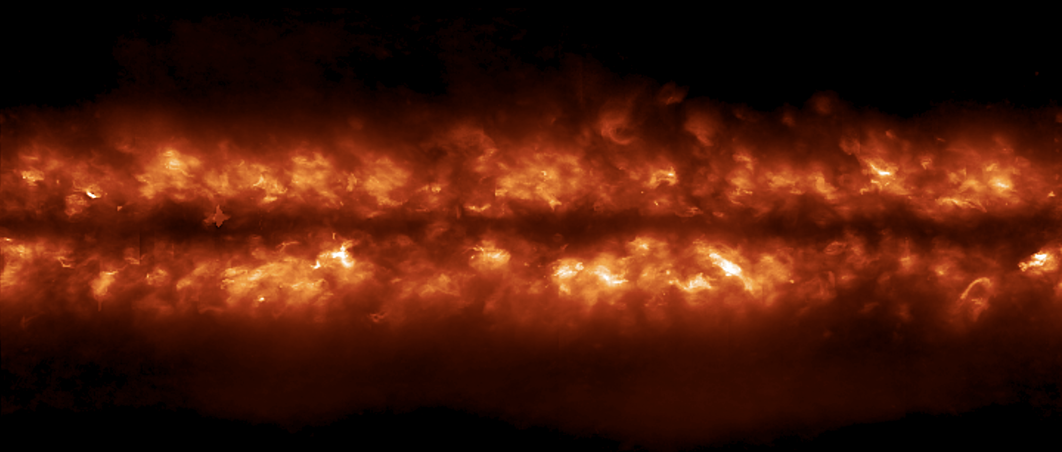
Cycle 24 Average Carrington Map
